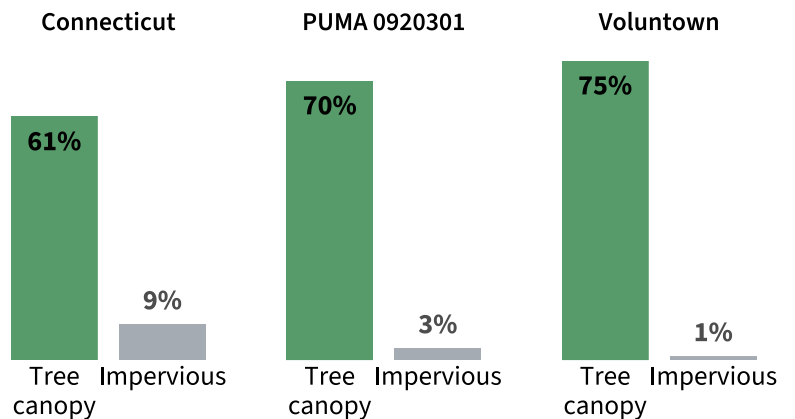
FIGURE 24: SHARE OF LAND BY LANDCOVER TYPE
